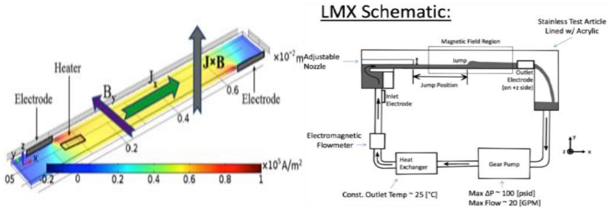
Figure 5: Schematic of the LMX, showing the capability to apply various electromagnetic fields and heat. The flow loop (galinstan) is shown in the panel on the right.
