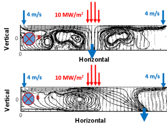
Figure 2: MHD/heat transfer analysis for the shallow tub-like Li divertor based on the Q2D flow model [37]. The figure shows the locations of the incoming IB and OB jets, drain orifice, applied heat flux and the computed flow field in the liquid for two configurations: (a) the drain is at the middle of the pool, and (b) shifted in the radially outward direction to x = 1 m.
