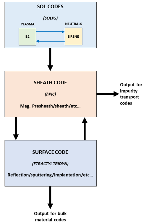
Figure 4: Flow chart of the plasma-surface modelling effort that will be used for plasma-interface modelling.
