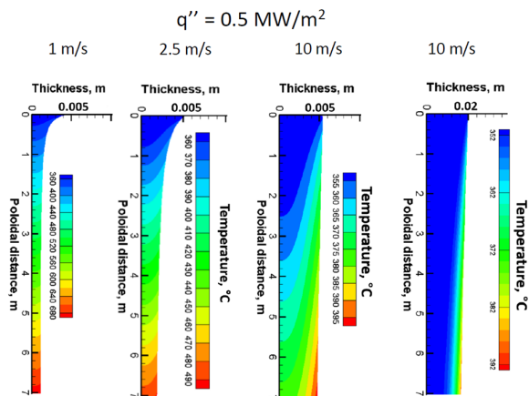
Figure 1: Example of 2D LM flow simulations for a give heat flux and varying flow speed and LM layer thickness, indicating a range of substrate participation in heat transfer [37].
