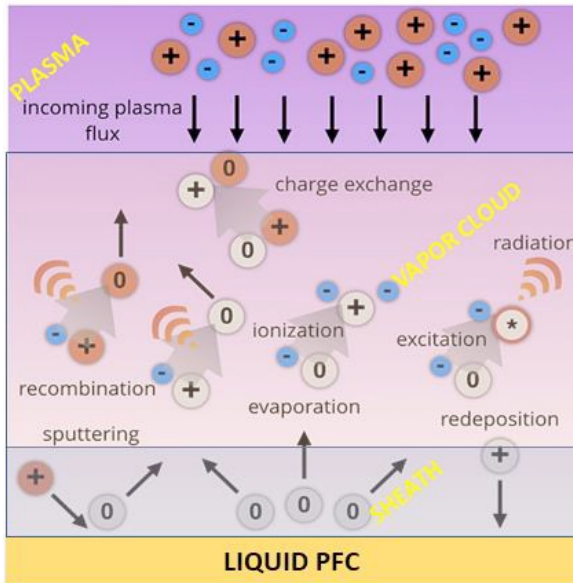
Figure 3: Behavior of ions and neutrals at the Liquid Metal / Plasma / Gas interface is important to accurately predict losses and ability to dissipate heat, etc. Graphic shows physics processes that need to be considered, e.g. sheath formation, sputtering, evaporation, adatom effects, ionization, re-deposition, migration, surface contamination, etc.
